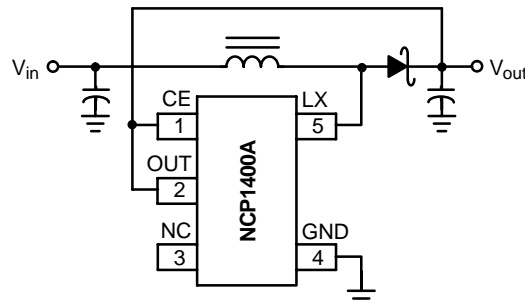
Figure 1. Typical Step-Up Converter Application
